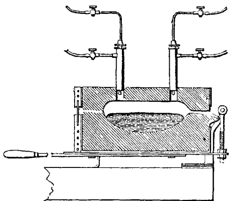
The lime-block furnace designed by Deville
