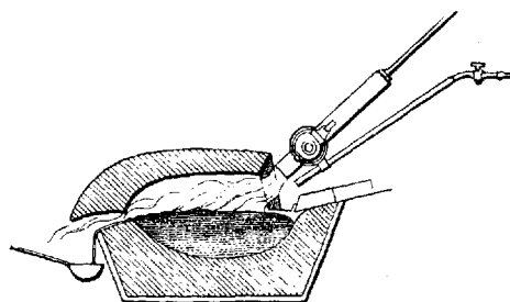
Removing the litharge in a fused state from the surface of the molten platinum
